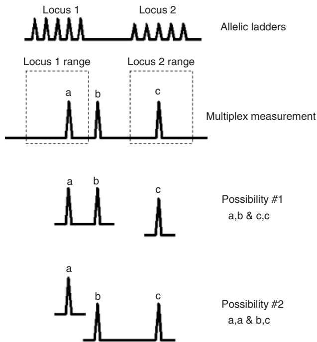
FIG. 1—Illustration of an interlocus allele observed in a measurement involving multiplex amplification where it becomes difficult to assign allele "b" to locus 1 or locus 2.
